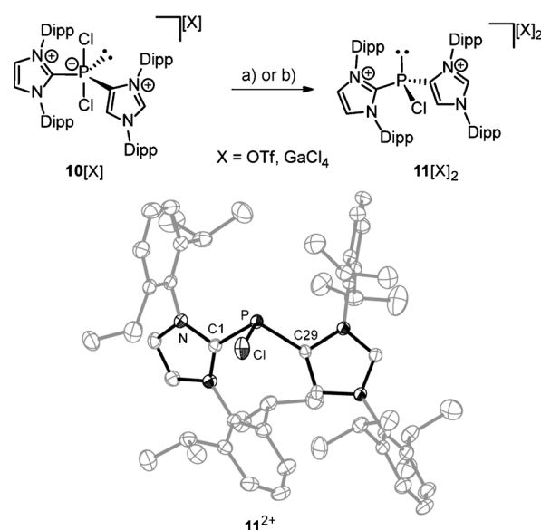
Scheme 3. Preparation of 11[X]_2 (top, a) ( X = OTf ) + \text{Me}_3\text{SiOTf} , -\text{Me}_3\text{SiCl} , \text{CH}_2\text{Cl}_2 , RT, 14 h, 95%; b) ( X = \text{GaCl}_4 ) + \text{GaCl}_3 , \text{CH}_2\text{Cl}_2 , RT, 14 h, 98%) and molecular structure of cation 11^{2+} (bottom, hydrogen atoms, solvent molecules, and anions are omitted for clarity, and thermal ellipsoids are displayed at 50% probability). Selected bond lengths [Å] and angles [°]: P1–Cl1 2.0458(1), P1–C29 1.820(2), P1–Cl1 1.838(3); C1–P1–C29 106.62(1), C1–P1–Cl1 100.24(8), C29–P1–Cl1 97.59(8).
