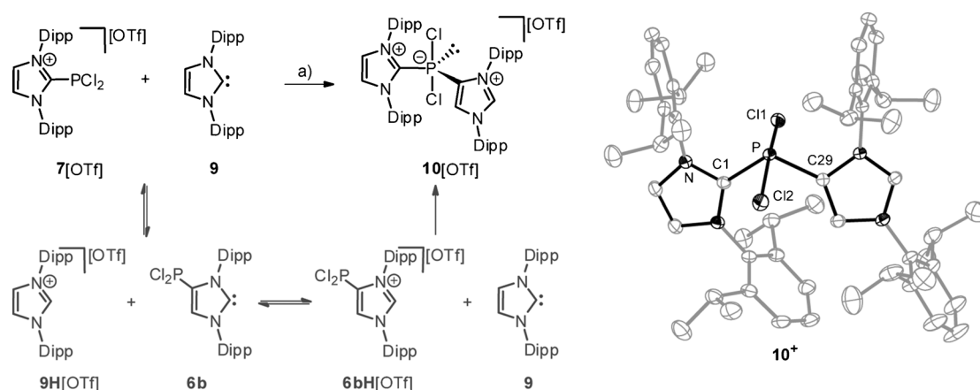
Scheme 2. Preparation of 10[OTf] (left, a) o\text{-C}_6\text{H}_4\text{F}_2 , -35^\circ\text{C} , 3 h, RT, 14 h, 96%), proposed reaction sequence for the formation of 10^+ (left, grey) and molecular structure of cation 10^+ (right, hydrogen atoms, solvate molecules, and anion are omitted for clarity, and thermal ellipsoids are displayed at 50% probability). Selected bond lengths [Å] and angles [°]: P1–C1 1.8679(2), P1–C29 1.8509(2), P1–Cl1 2.3135(6), P1–Cl2 2.3037(6); Cl1–P1–Cl2 166.9(2), C1–P1–C29 113.47(7), C1–P1–Cl1 84.02(5), C29–P1–Cl1 86.77(5), C1–P1–Cl2 87.27(5), C29–P1–Cl2 87.78(5).
